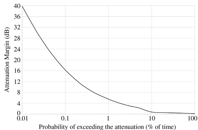
Fig. 3. Estimated total attenuation statistics for Salerno.
